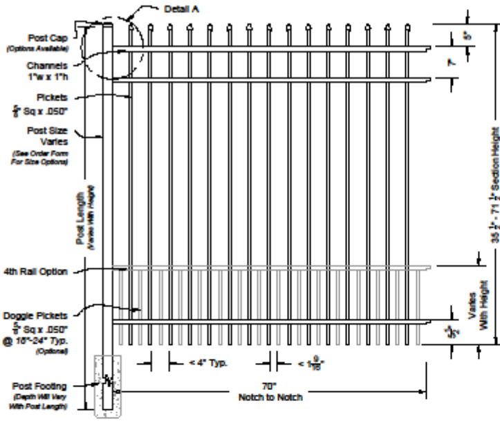
i 01 Maine #203 6ft Fence Panel Shown As Residential Series Scale: NTS
